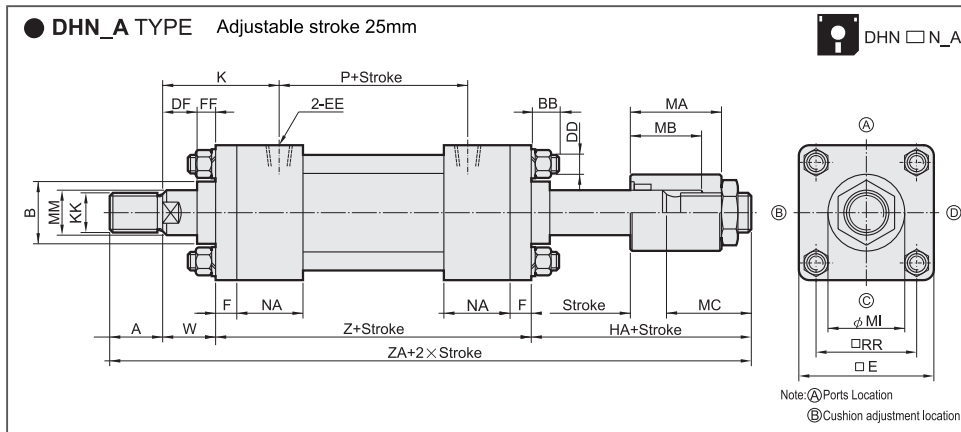
Dimensional Table
