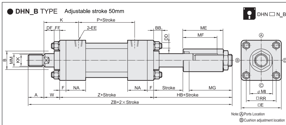
Dimensional Table
