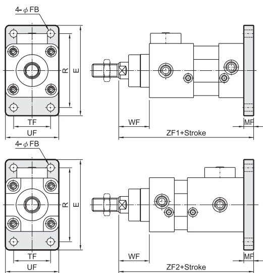
Dimensional Table
