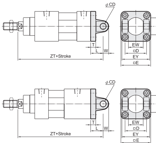
Dimensional Table
