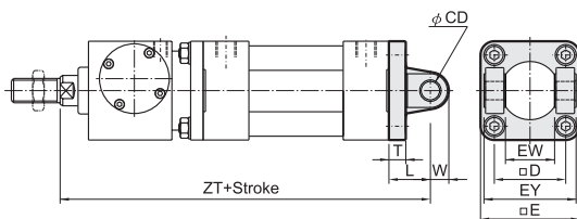
Dimensional Table
