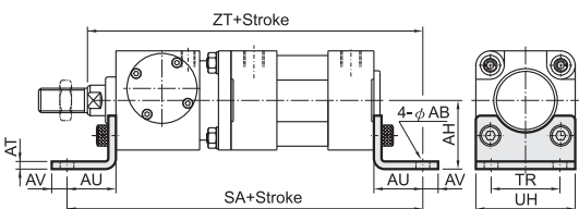
Dimensional Table
