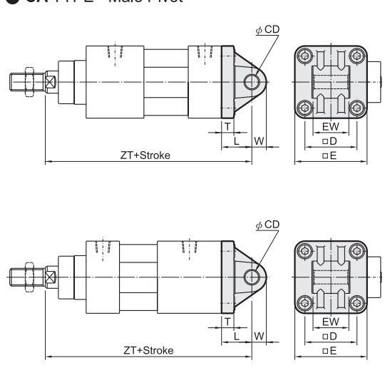
Dimensional Table
